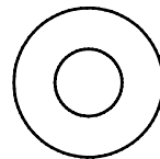
(C5) 5/16" (I.D.) FLAT WASHER \varnothing 18 QTY.7
